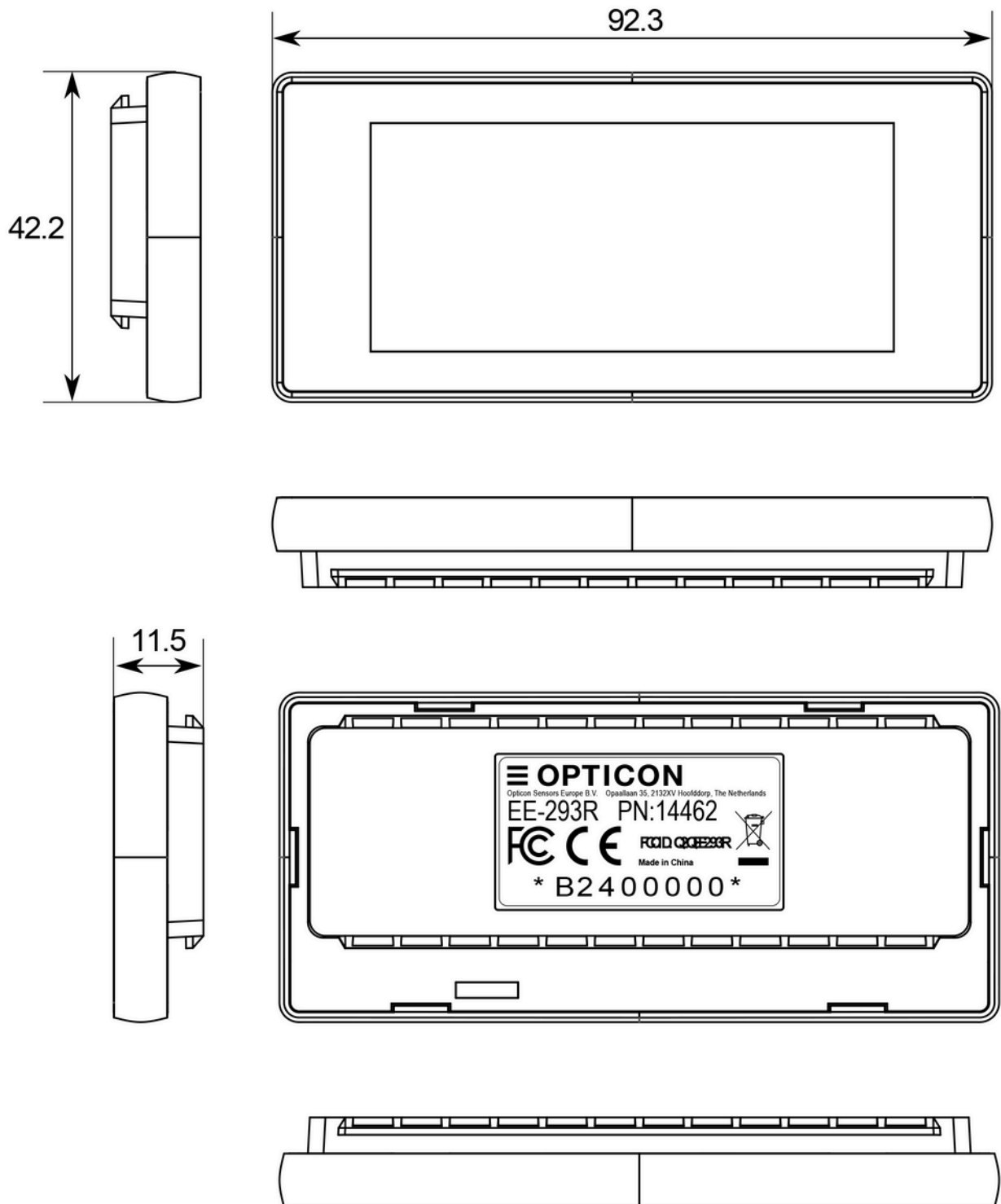
Figure 8: Mechanical drawing
